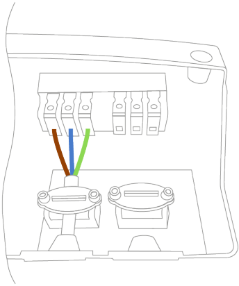
Backup connection terminals
