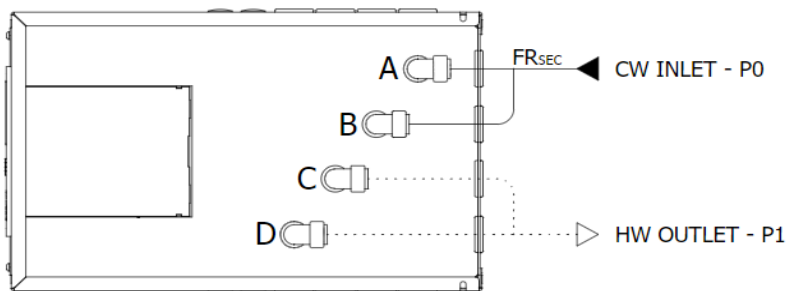
Figure 6.6: Pressure loss at inlet & outlet of the UniQ eHW 12 +iPV
