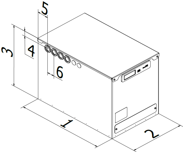
Figure 5: Additional Sunamp Ltd UniQ (e)HW +iPV Heat Battery dimensions
