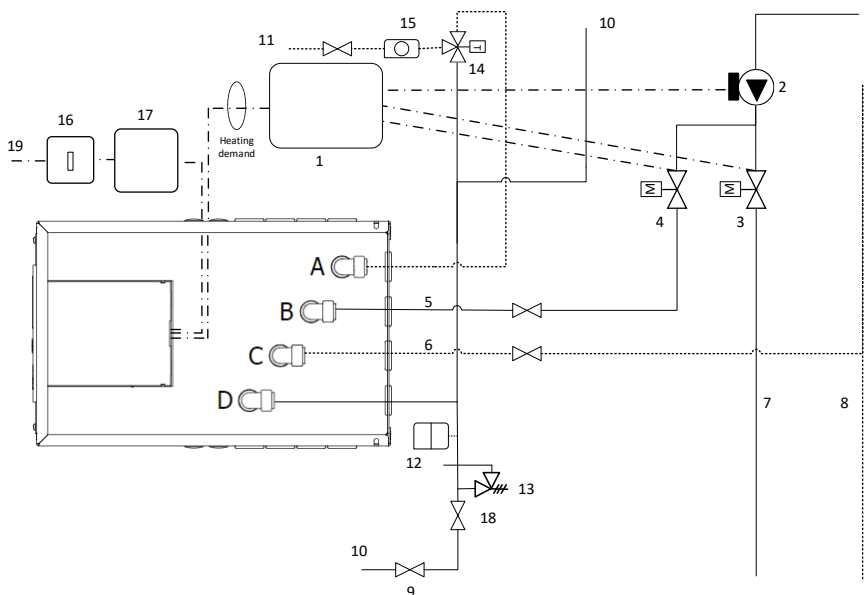
Figure 14. 1: Example wiring option 1 schematic (see Figure 3a for piping and electrical options available)
