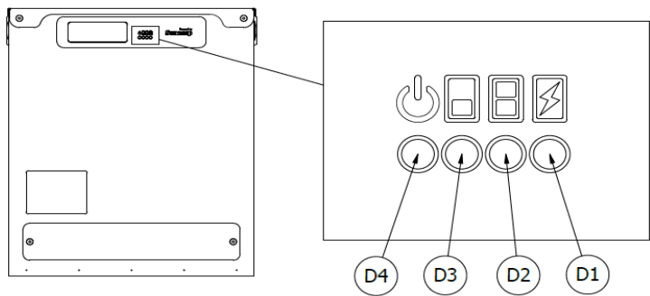
Figure 4: LED interface
