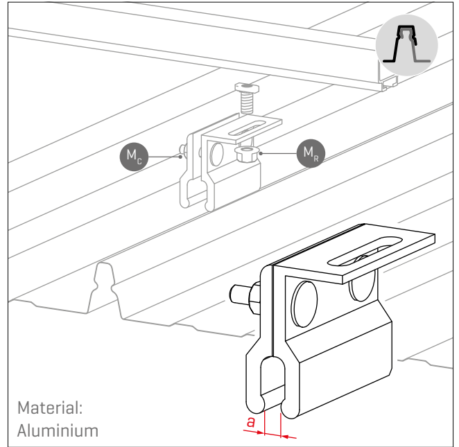
Rib-Roof 465 Clamp 2002118
