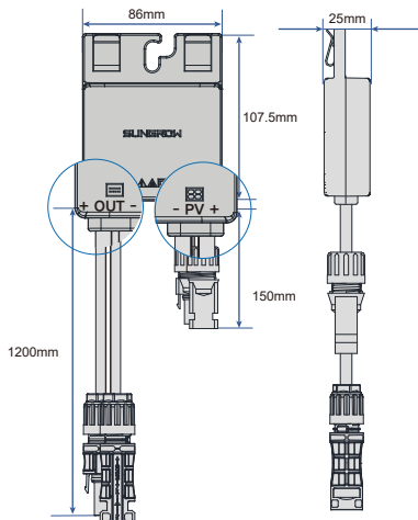
Short PV wire version:
