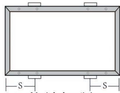
Module length L Mounting by clamps ( S=1/4L\pm 50 )
