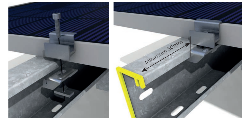
Fig.12– End clamp install (caphead & swingnut shown)
