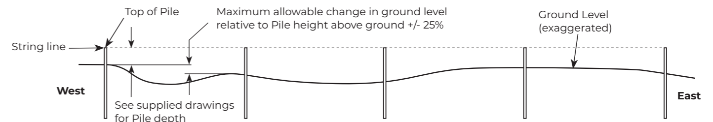
Fig. 15 – Setting out of pile heights
