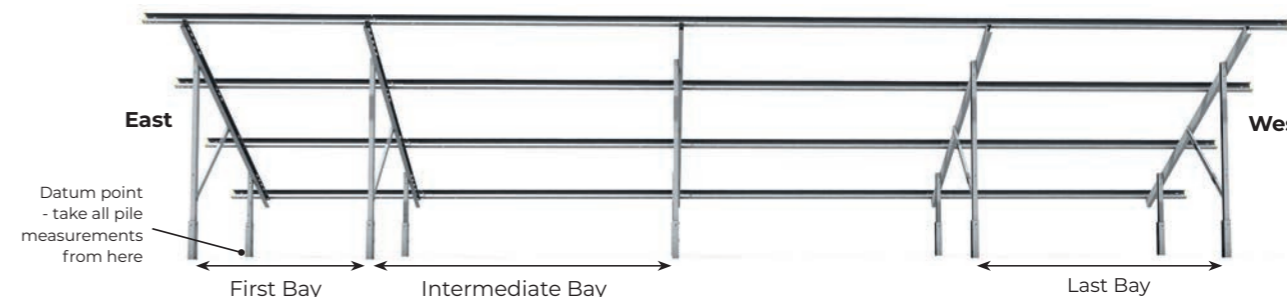
Fig.3 - Setting out (viewed facing south)
