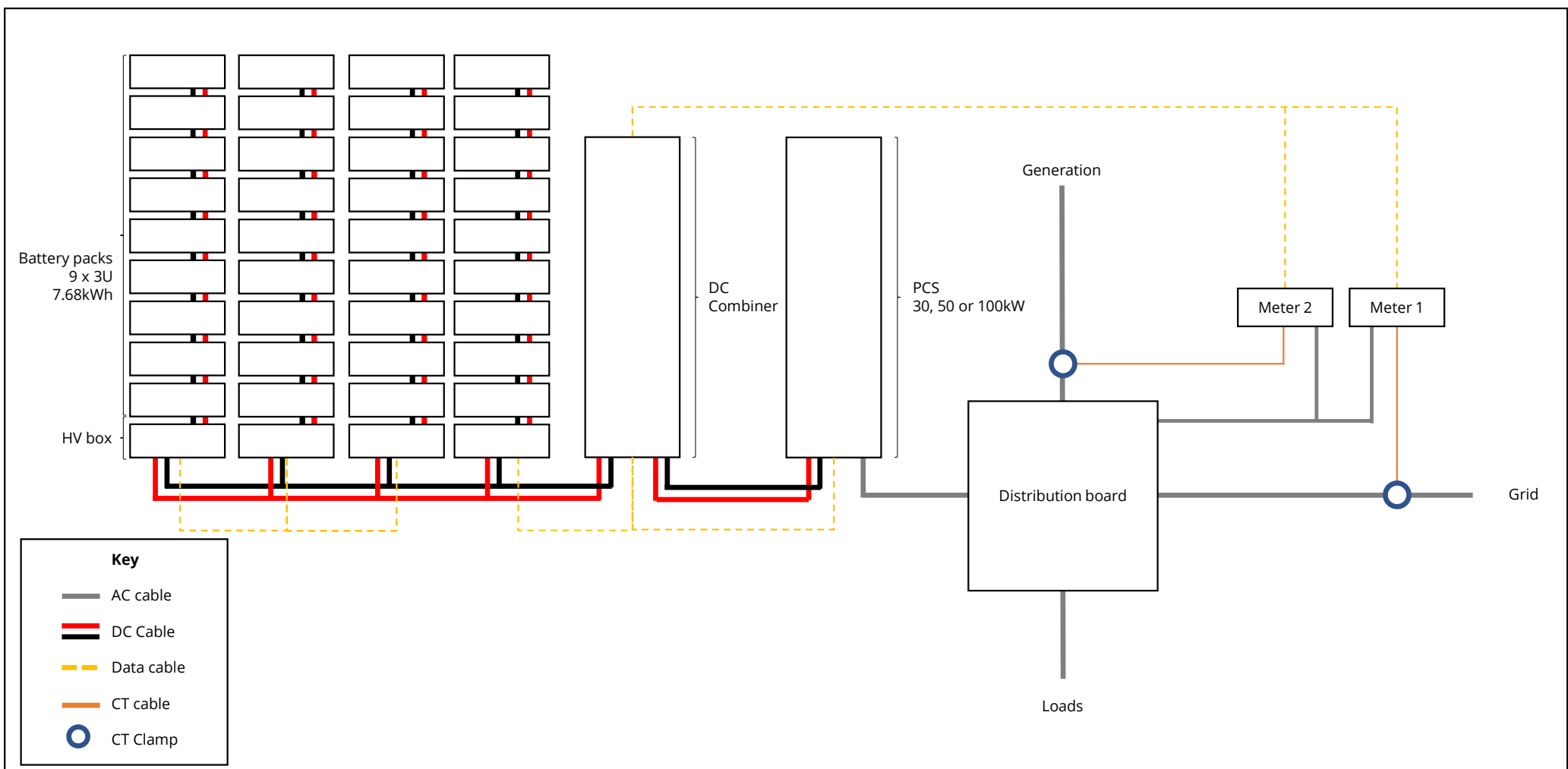
SME 276kWH Sample Wiring Schematic
