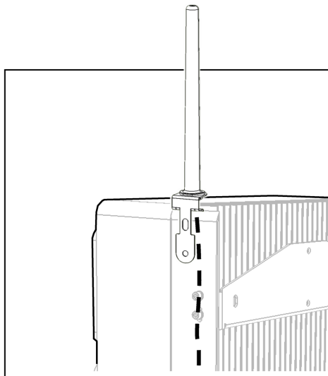
Figure 10: Mounting the Antenna
