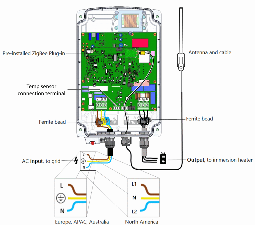
Figure 9: Smart Energy Hot Water wire connections
