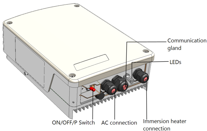
Figure 3: Device interfaces
