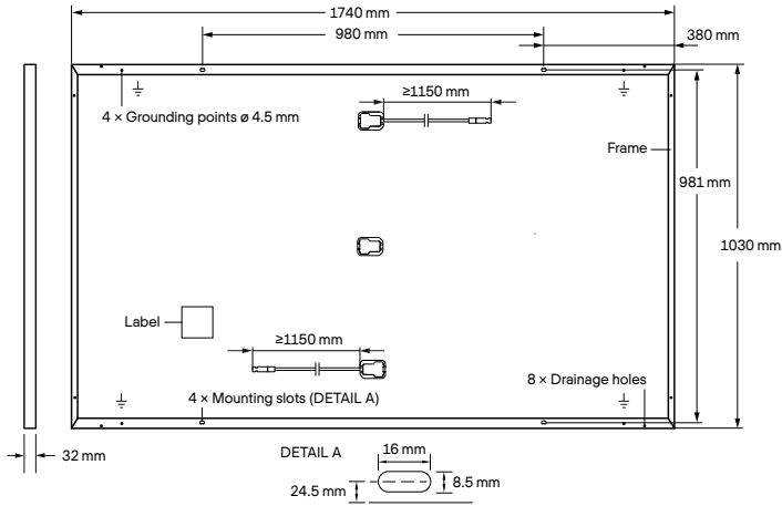
Fig. 1: External dimensions and components for Q.PEAK DUO-G8, Q.PEAK DUO-G8+, Q.PEAK DUO BLK-G8 and Q.PEAK DUO BLK-G8+
