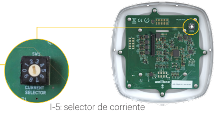
I-5: selector de corriente
