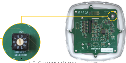
I-5: Current selector
