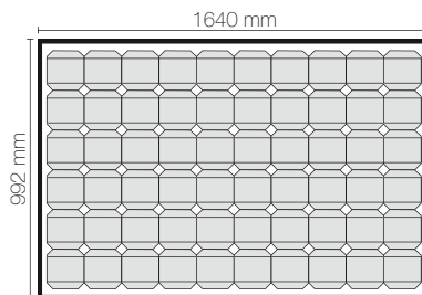
PLM-250P-60 Series/ PLM250PB-60 Series Weight: 18kg
