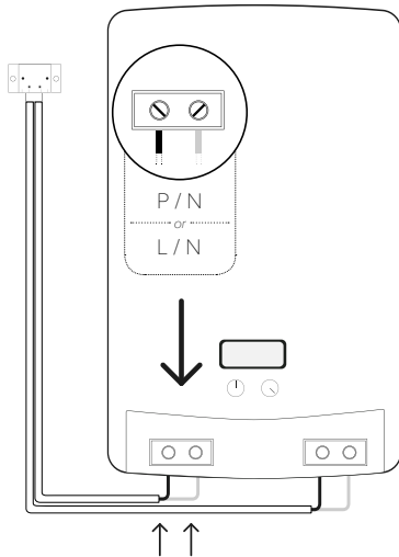
230 V Power supply terminals Blue and brown wires
