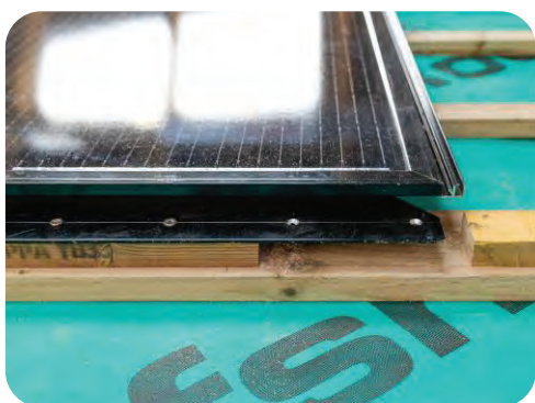
B: Cut out 200mm of top batten from RHS outside edge of panel
