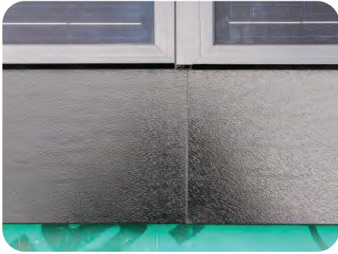
E: Push bottom flashing together
