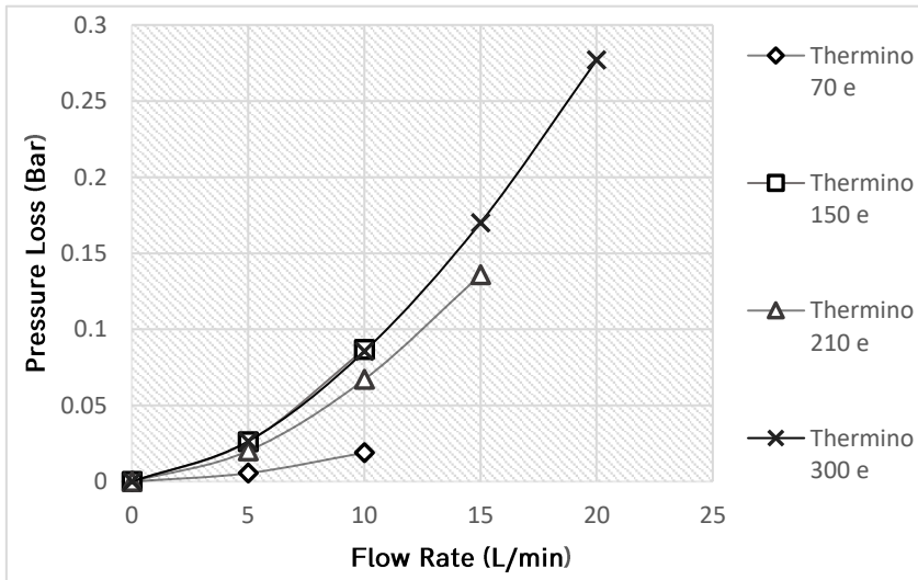
Figure 3 – Thermino ePlus Heat Batteries pressure loss
