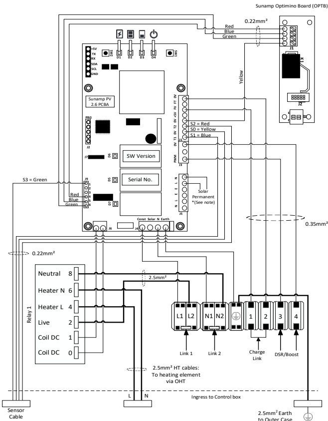
Figure 9 - Thermino ePlus Heat Battery wiring overview
