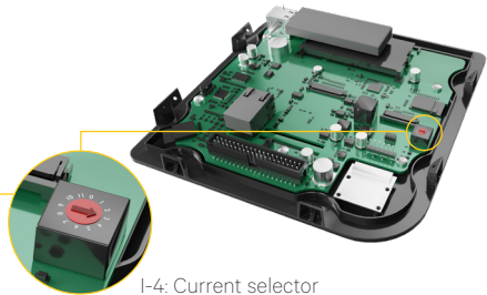
I-4: Current selector
