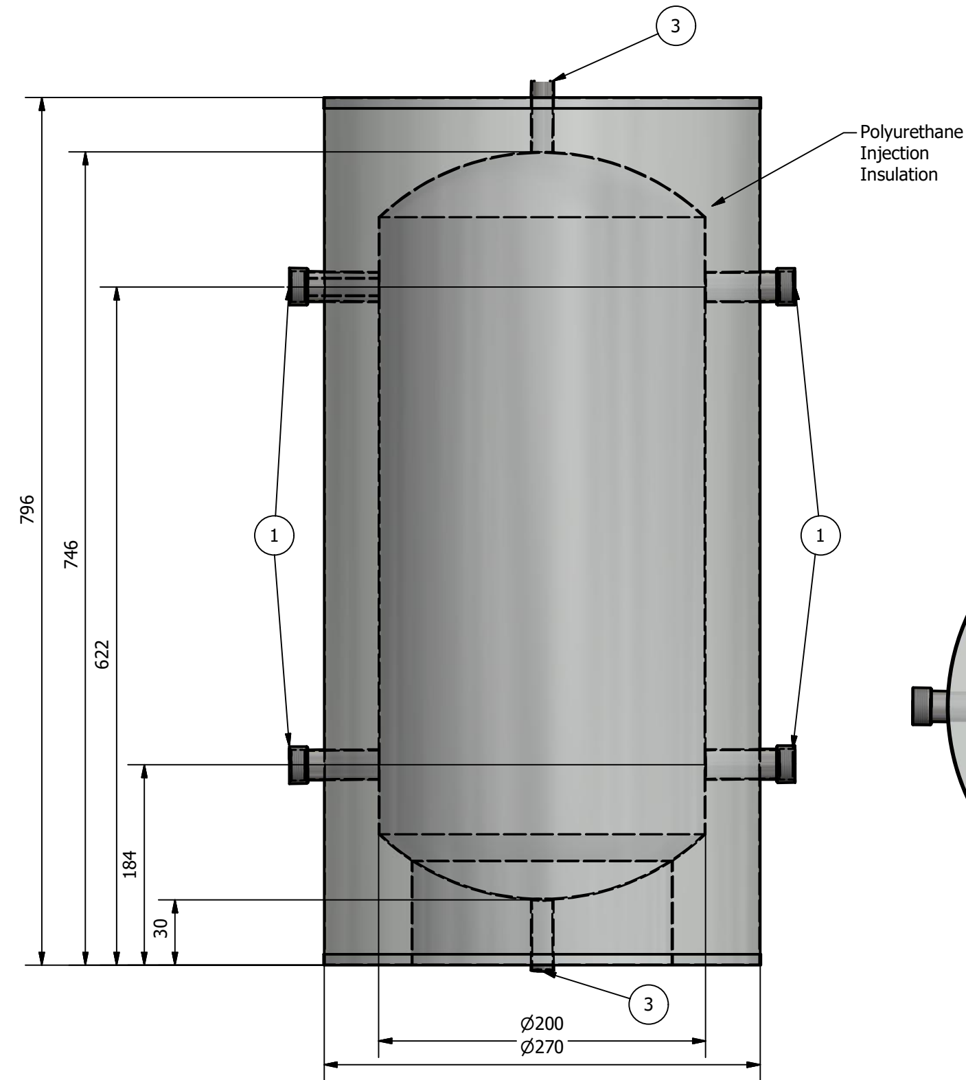
Front View (0.21 : 1)
