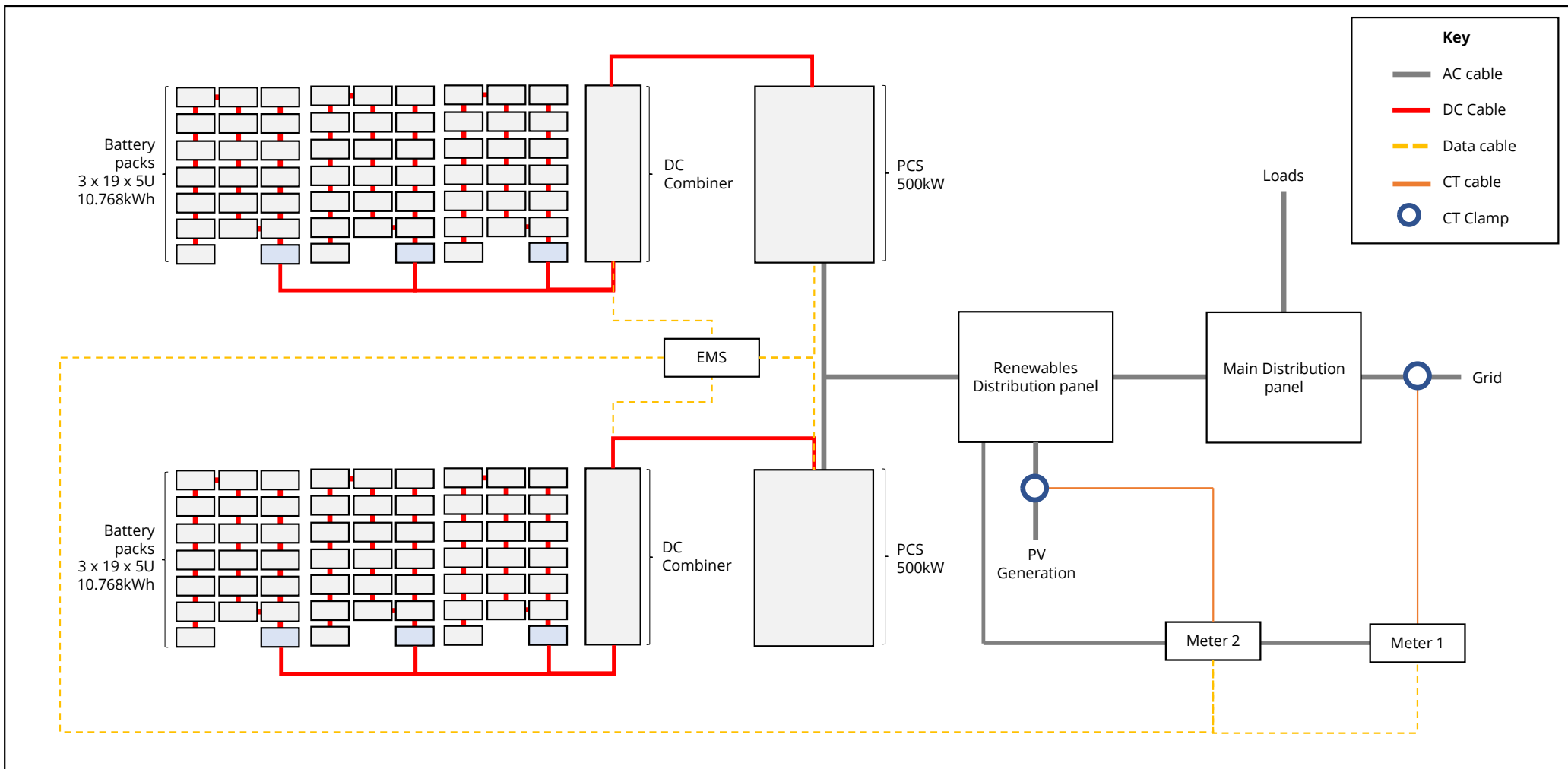
SME 1.2MWH/1MW Sample Wiring Schematic
