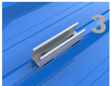
Fasten the mini rails with metal sheet roof with 2pcs of rubber pads and 2pcs st6.3*25 tapping screw.
