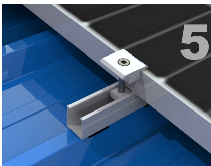
Install the mid clamps with mini rail.
