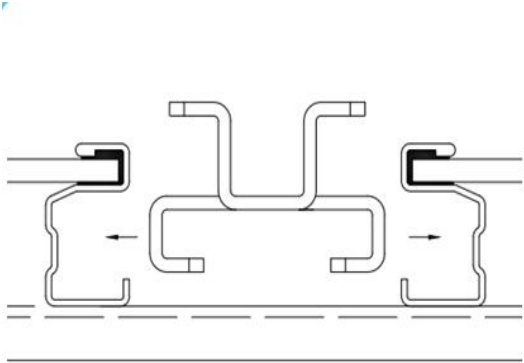
1.Insert the tongue of the mid clamp into the cavity of the steel frame
