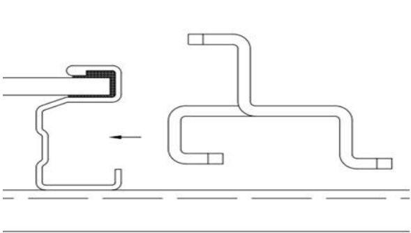
1.Insert the tongue of the end clamp into the cavity of the steel frame
