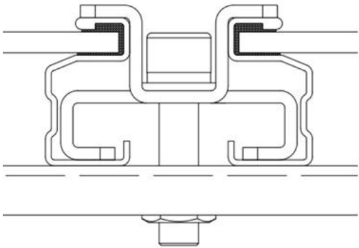
3.Schematic diagram of completed installation
