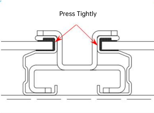
2.Press the left and right vertical faces of the clamp tightly against surface B of the frames
