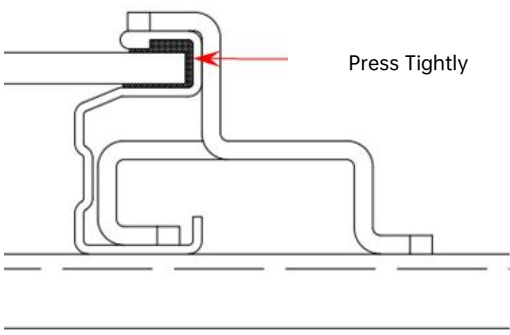
2.Press the vertical face of the clamp tightly against surface B of the steel frame
