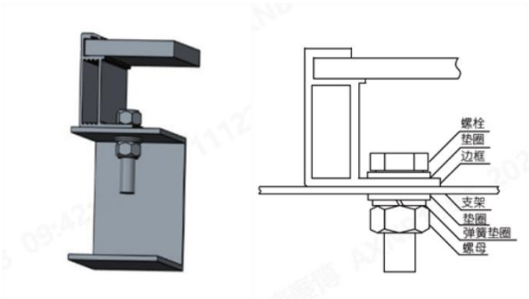
Bolts mounting of anodized aluminum frame
