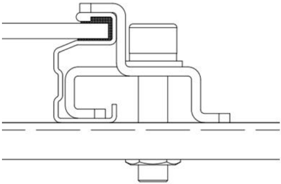
4.Schematic diagram of completed installation
